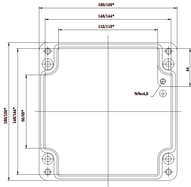
Deckel
