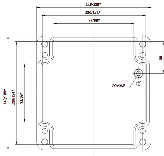
Deckel
